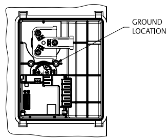
TERMINAL BOX LAYOUT STANDARD SCALE 2:3
