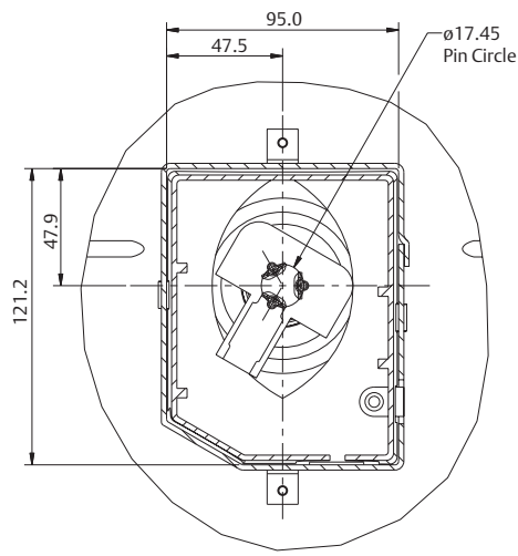
T-Box Layout Standard Section A-A Scale 1:1
