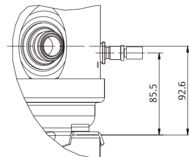
Detail VALVE Scale 3:4
