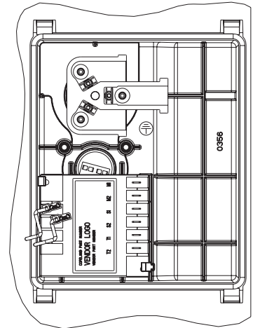
Terminal Box layout Standard © Scale 3:4
