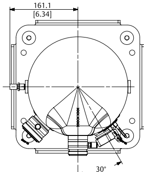
SIGHT GLASS VIEW
